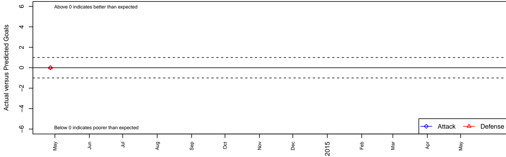
Xolos Academy B95 Dots are actual minus expected GF (blue circles) and GA (red triangles). Blue line is smoothed change in attack strength. Red is smoothed change in defense strength.
